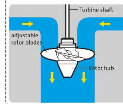
Kaplan turbine
